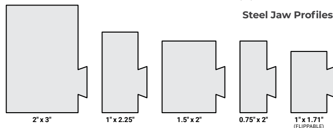
Aluminum Jaw Profiles
