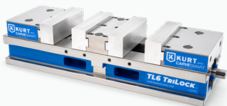
TL6CSP with 6-inch extruded aluminum jaws
